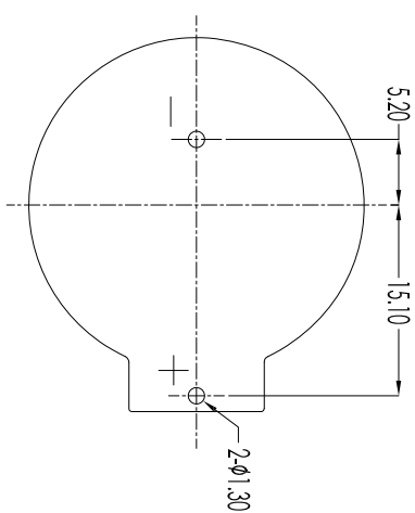
PCB Layout Diagram Top View
