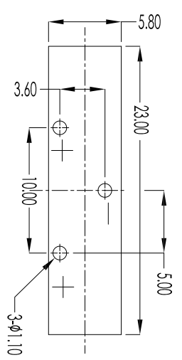
PCB Layout Diagram Top View
