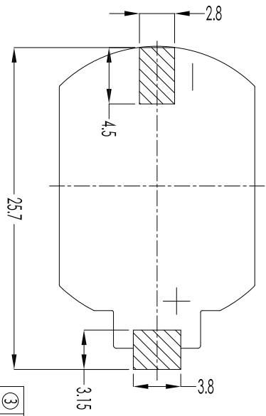
PCB Layout Diagram Top View
